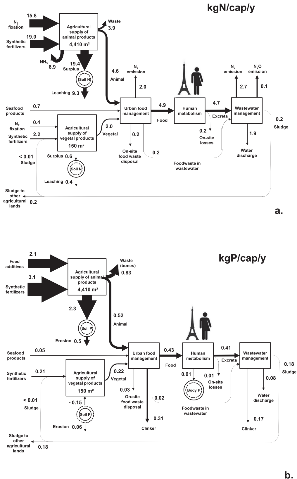
Fig. 8. Summarized representation of the nitrogen (a) and phosphorus (b) imprint of human metabolism in Paris Megacity. The flows are expressed in kgN or kgP per capita and per year.
