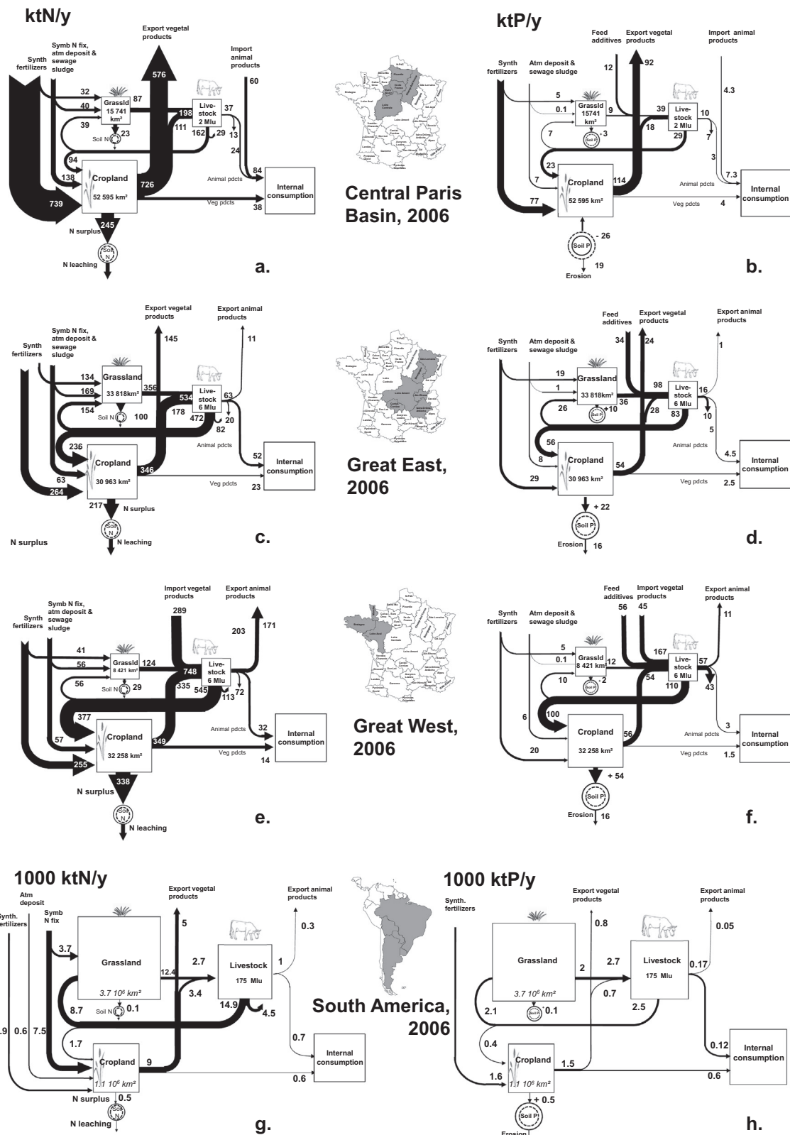
Fig. 4. Generalized Representation of the Agro Food System (GRAFS, Billen et al. 2014), in terms of N fluxes (a, c, e and g) and P fluxes (b, d, f and h) between cropland, grassland, livestock and local human consumption. The N- and P-GRAFS have been established for the 4 main areas contributing to Paris Megacity food supply: Central Paris Basin (a and b), Great East (c and d), Great West (e and f) and South American soy exporting countries (g and h).
