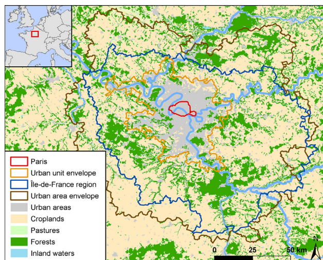
Fig. 1. The perimeters of the Paris city center, urban unit, urban area and Ile-de-France administrative region. The background shows the main types of land use (from European Environment Agency, 2013).
