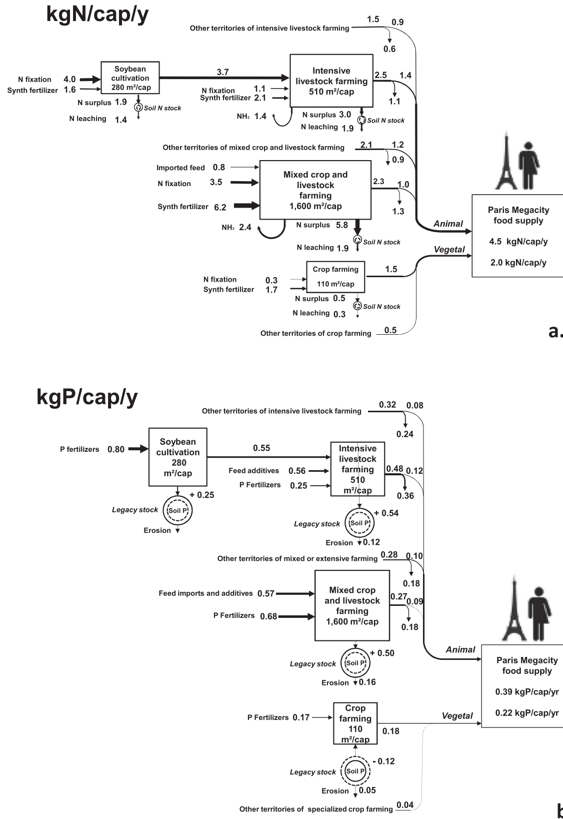
Fig. 5. Flows of nitrogen (a) and phosphorus (b) which can be attributed to the food supply of one inhabitant of Paris Megacity in the different agricultural areas involved. The flows are expressed in kgN or kgP per capita and per year.
