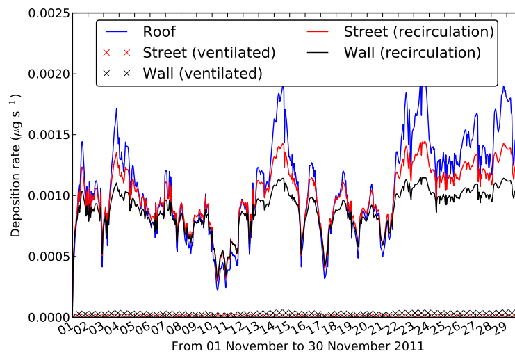
FIGURE 4.11 – Deposition rate ( \mu\text{g s}^{-1} ) of pollutants ( \bar{c} = 1 \mu\text{g m}^{-3} ) for each surface and region in November 2011.
