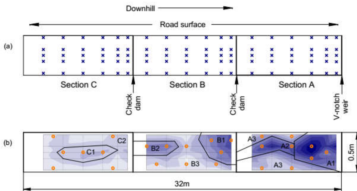
Figure 82: Schematic of (a) surface soil sampling and (b) core sampling the biofiltration swale in Compans. Surface samples were taken at every node of the grid (a), while cores were taken at each orange circle and mixed according to zones (A1, A2,A3, B1, B2,B3 and C1, C2) selected based on the cartography of copper concentrations shown in the background (b). Please note that horizontal and vertical scales are different.
