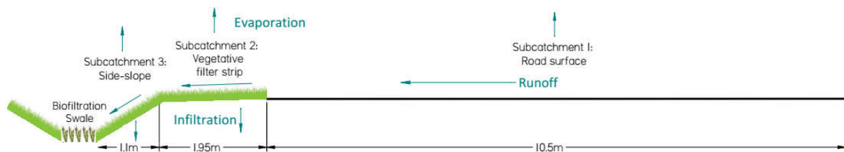
Figure 23 : Geometry of the modeled system
