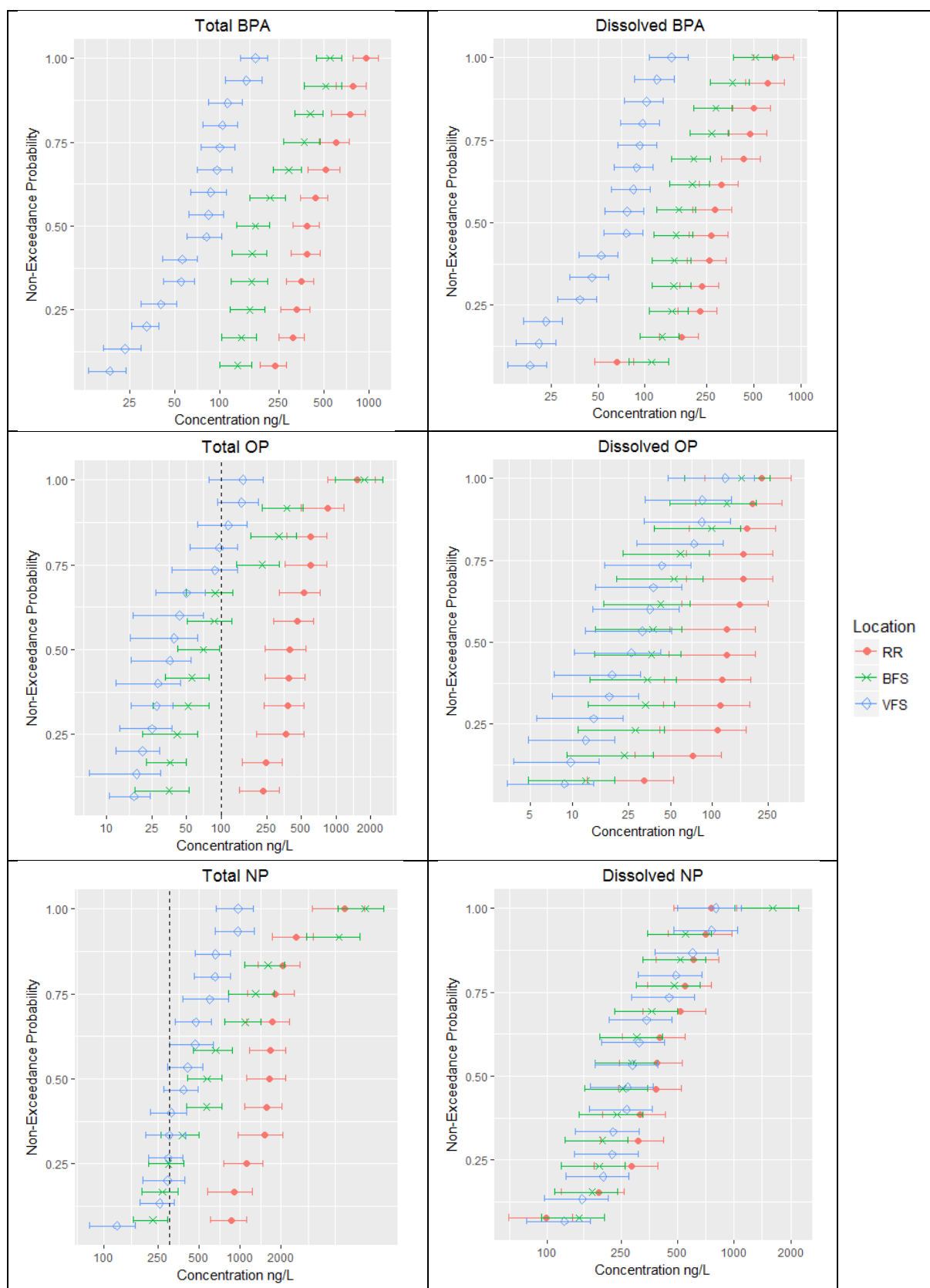
Figure 54 : Probability distribution of total and dissolved BPA, OP and NP in road runoff (RR), the vegetative filter strip (VFS) and the biofiltration swale (BFS). Error bars represent analytical uncertainty while the dotted black line represents the EQS.
